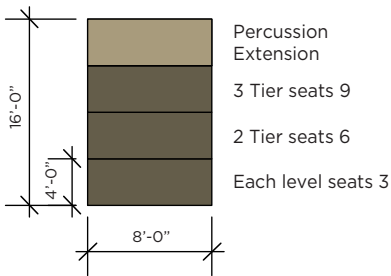
SB8 8' Straight Section
